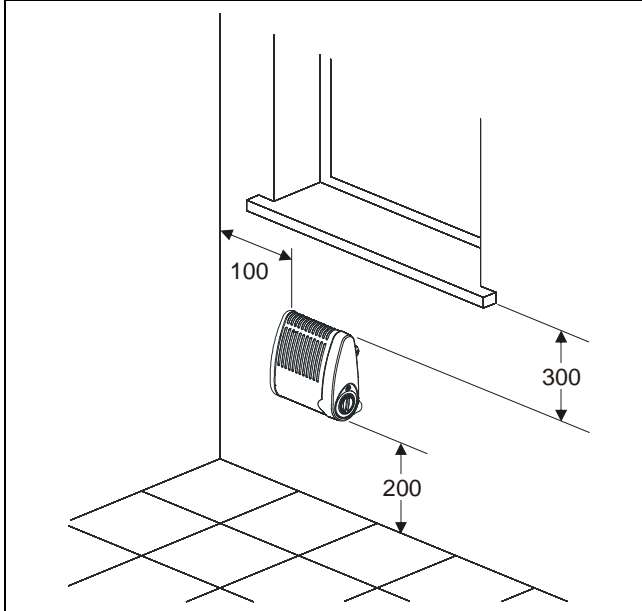
Fig. 1: Minimum clearance
