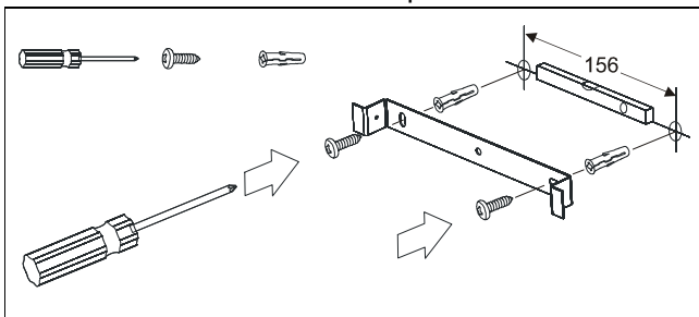
Fig. 2: Drill dimension
